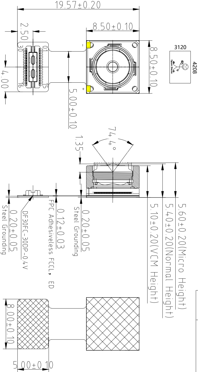
TOP VIEW
